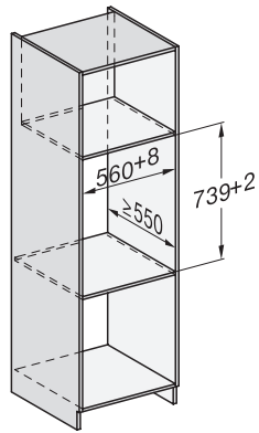
Installation DG, DGM, DGC XL, ESW7x20 installation drawings
