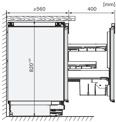
KU7030D, Built-under, side view
