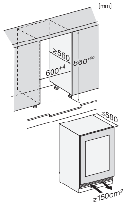
KWTUS7196E, Built-under, niche dimensions
