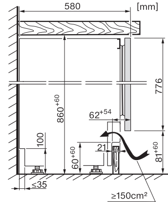
KWTUS7196E, Built-under, side view
