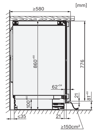
KWTUS7196E, Built-under, side view
