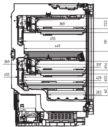
KWTUS7196E, interior dimensions
